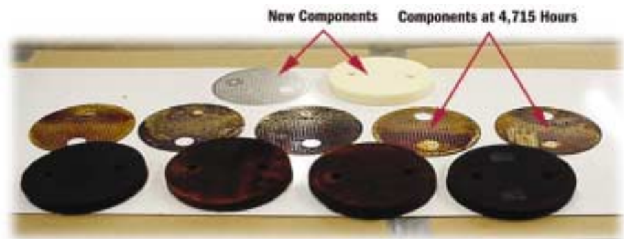
Figure 1. New and Used Electrostatic Cell Components
