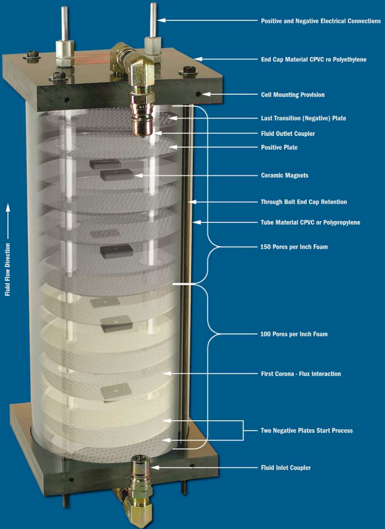
Figure 2. Electrostatic Cell Construction
