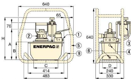
ZA4-Series Pumps with 4 - 6,6 litres reservoir
