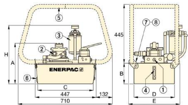
ZA4-Series Pumps with 10, 20 and 40 litres reservoir
