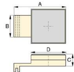
ELP-60, ELP-80 Levelling Plate
