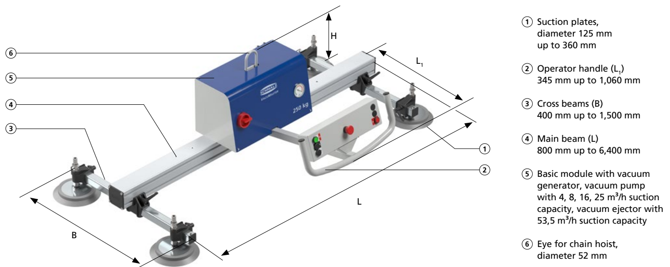
Fig. shows VacuMaster Comfort
