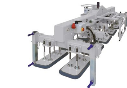
Special VacuMaster Vario with lift capacity of 10 t (special applications with lift capacity over 2 t on request)
