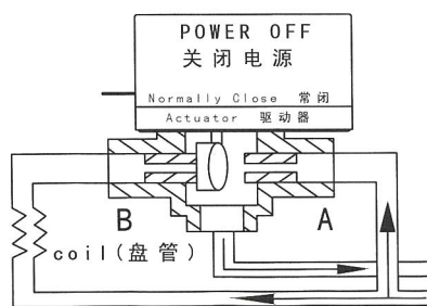
Fig. 4: 3-way valve in Mixing Configuration, Normally Closed to coil 图 4: 三通阀混合布置(常闭)管道安装
