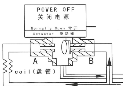
Fig. 3: 3-way valve in Mixing Configuration, Normally Open to coil 图 3: 三通阀混合布置(常开)管道安装
