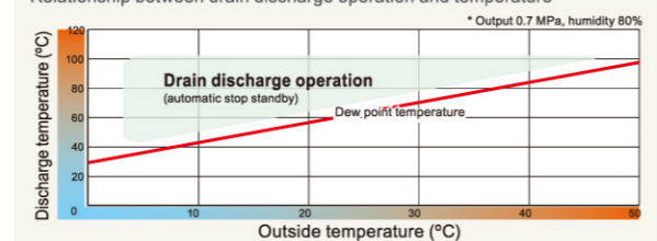
Relationship between drain discharge operation and temperature
