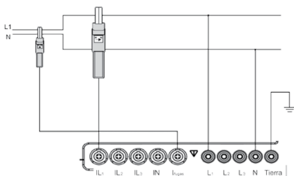
Single-phase system
