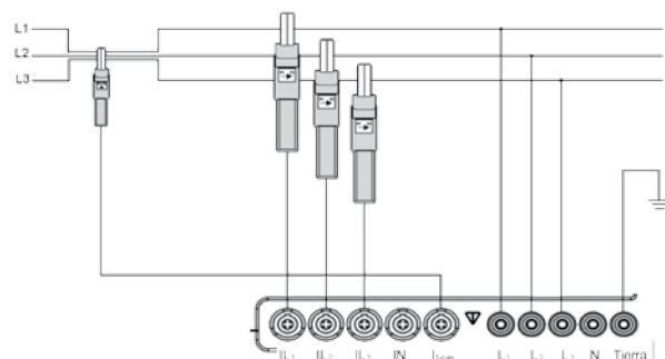
Three-phase system without neutral
