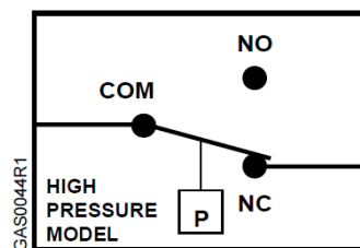
Figure 2. Typical Wiring for High Pressure Models.
