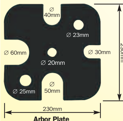
Arbor Plate
