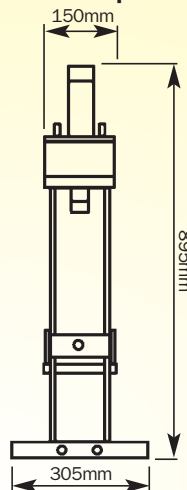
Ram Adaptor
