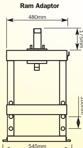
Ram Adaptor
