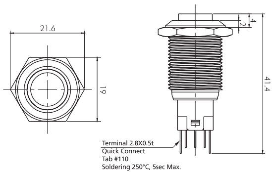
LED Illumination Push Button Switch (Extended)
