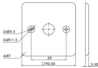
T - P2 (Ø19 only)
