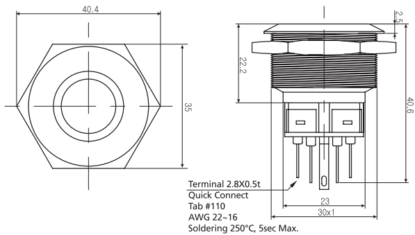
LED Illumination Push Button Switch (Flush)
