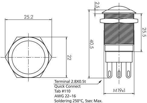
Non-Illumination Push Button Switch (Dome)
