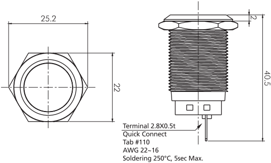
LED Pilot lamp (Flush)
