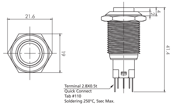
Non-Illumination Push Button Switch (Extended)
