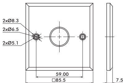
T - P1 (Ø19, 22, 25, 30)
