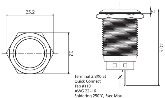
LED Illumination Push Button Switch (Flush)
