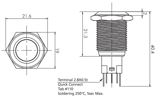
LED Illumination Push Button Switch (Flush)
