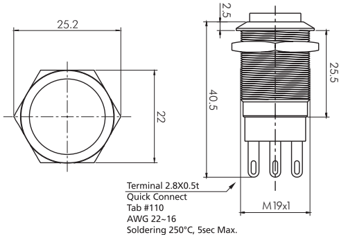
Non-Illumination Push Button Switch (Extended)
