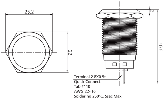
Non-Illumination Push Button Switch (Flush)
