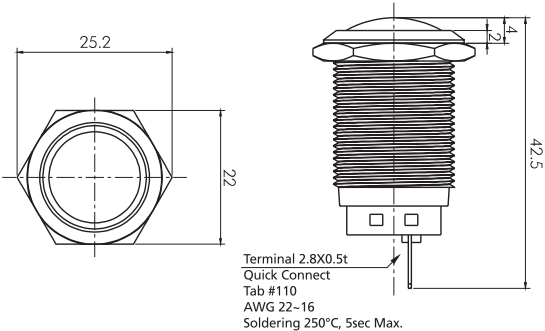
LED Pilot lamp (Dome)
