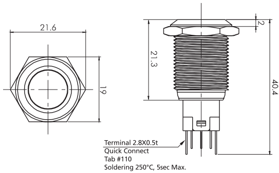
Non-Illumination Push Button Switch (Flush)
